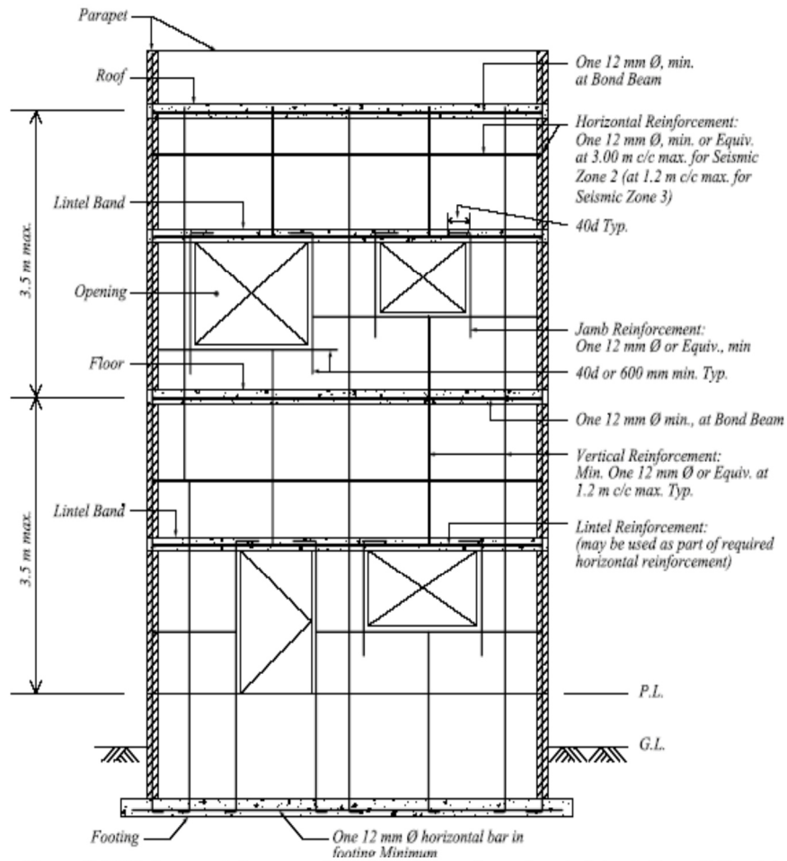
Figure 6.7.2 Typical details of vertical reinforcement in hollow block masonry
